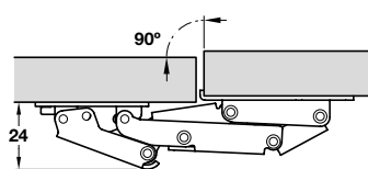
Flap open
