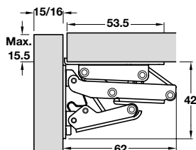
Flap closed
