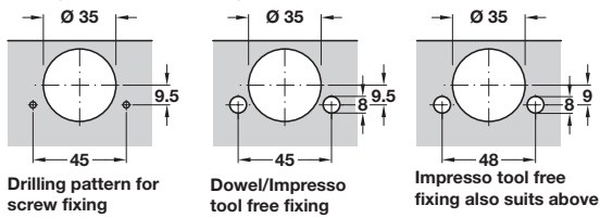
Drilling pattern for screw fixing
