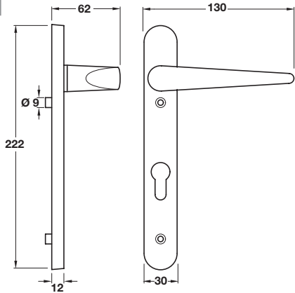
Backplates for euro profile cylinder multi-point lock
