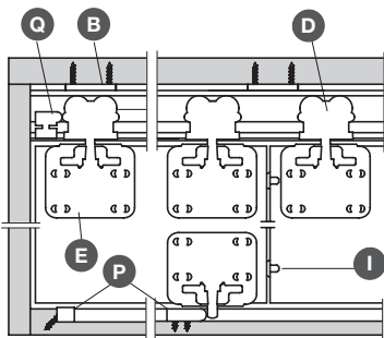
Detail of door closing off storage area
