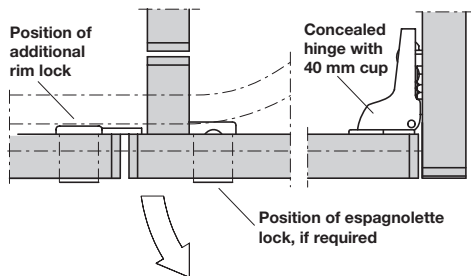
Detail of door closing off storage area
