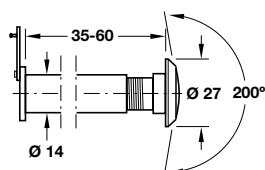
To suit doors 35-60 mm thick
