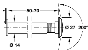
To suit doors 50-70 mm thick
