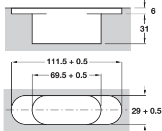
Frame and door drilling pattern
