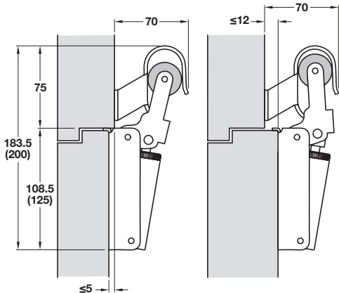
Specifications in brackets apply to soft closing mechanism for door weights 80 kg
