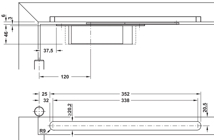
Door frame preparation details
