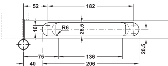
Door leaf preparation details
