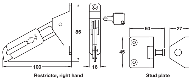
Restrictor, right hand
