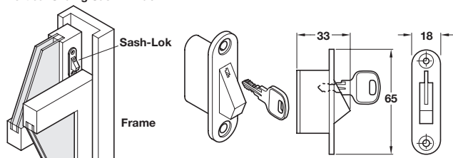
Vertical Sliding Sash Window
