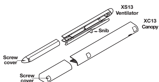
Slot detail and dimensions 411 mm long vent
