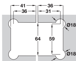
For 8/10 mm glass, with bulb seal Cat. No. 950.34.062
