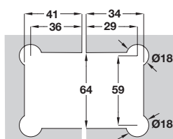
For 12 mm glass, with bulb seal Cat. No. 950.34.062
