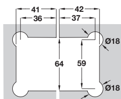
For 8/10 mm glass, without seal
