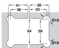
For 12 mm glass, with H-profile seal Cat. No. 950.34.042
