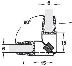
when used with 6 mm thick glass
