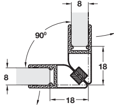
when used with 8 mm thick glass
