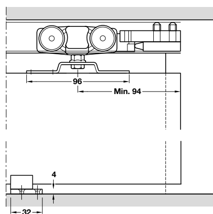
Section trolley hanger and guide
