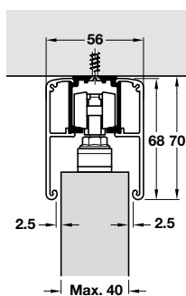
Ceiling installation
