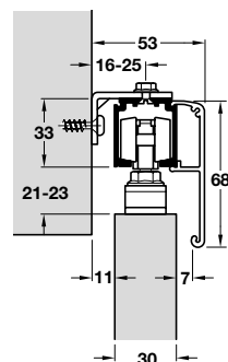
Wall mounted installation with clip panel and concealed mounting bracket
