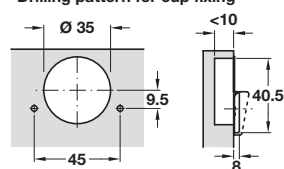
Drilling pattern for screw fixing
