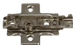
Cruciform mounting plate, 4 point fixing
