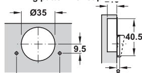
Drilling pattern for screw fixing
