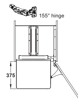
Cabinet clearance
