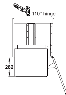
Cabinet clearance
