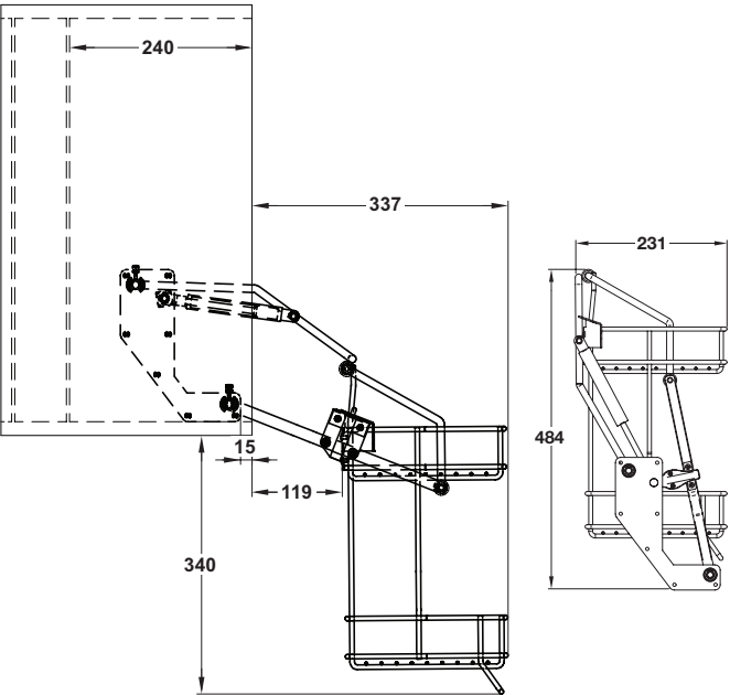
Pull down two tier wire shelf
