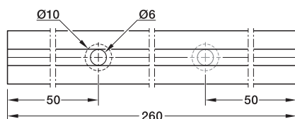
Example wall hanging drilling dimensions
