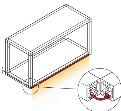
Installation of optional lighting
