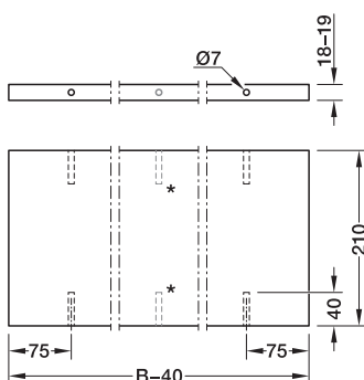
Shelf drilling dimensions
