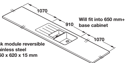
Sink module 1.5 bowl Stainless steel 3050 x 620 x 15 mm
