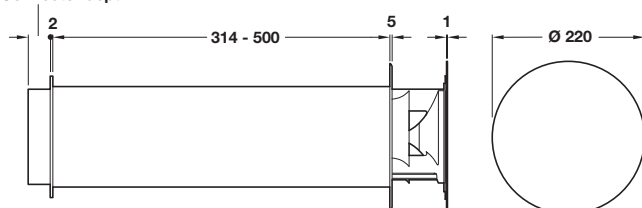
System 150: For installation in approx. Ø 155 mm hole
