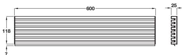
Fixing strip
