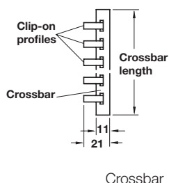
Quantity of clip-on profiles, determined by length of cross bar
