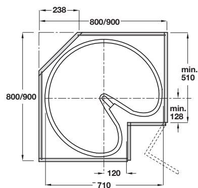
Ninka Pro(arc) three-quarter carousel set
