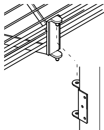
Pivot fixing bearing
