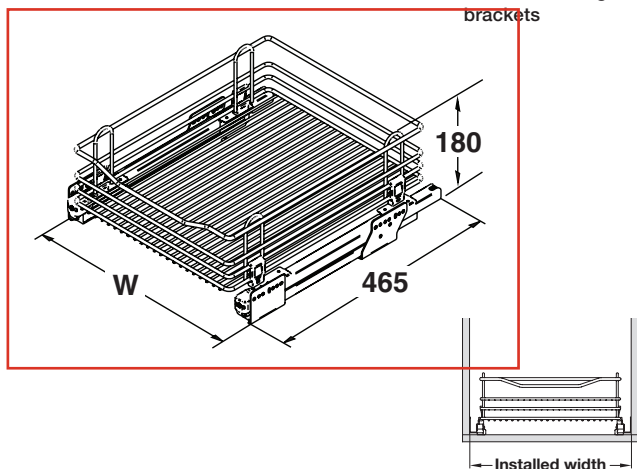
Door front fixing brackets
