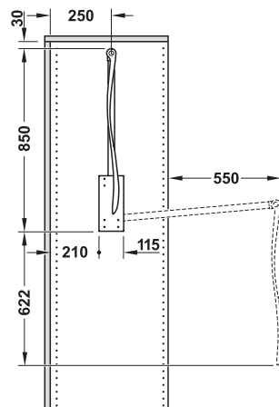
Installation in centre of cabinet side panel
