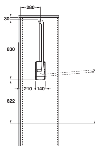
Installed in middle of cabinet side wall
