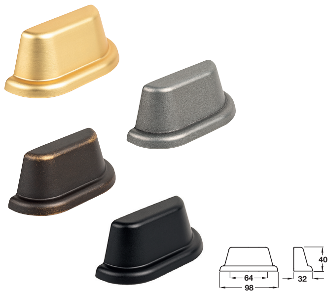
LAND cup pull handle
