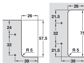
Screw fixing drilling diagram
