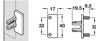
Dowel fixing
