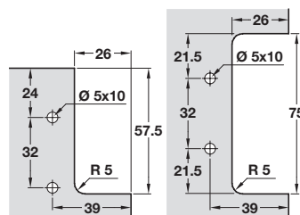
Dowel fixing drilling diagram
