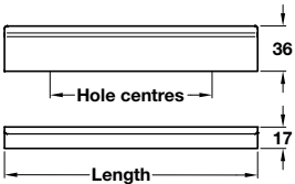
CURVE profile handle
