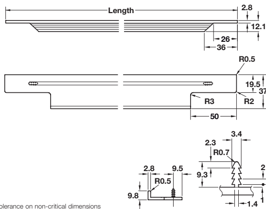
PORTOBELLO profile handle
