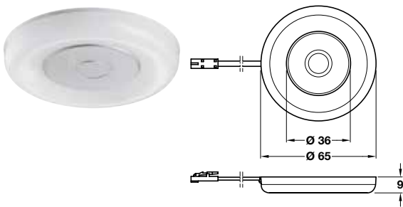
Loox5 12V LED 2027 downlight, Ø 65 mm
