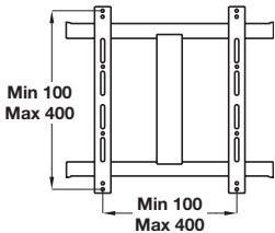
THIN 445: Extends up to 508 mm Wall bracket width x height: 52.5 x 232 mm
