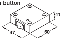
Push button
