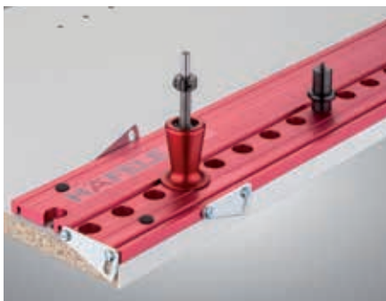
The drilling jig is moved and fixed with the locating pin for longer rows of series drilled holes
