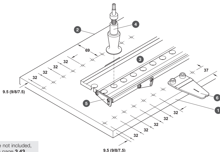
The drilling jig is moved and fixed with the locating pin for longer rows of series drilled holes
