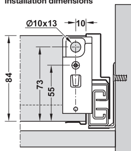
Rear wooden panel installation dimensions
