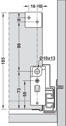
Rear wooden panel installation dimensions
