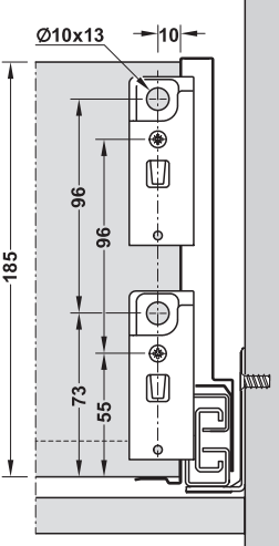
Rear wooden panel installation dimensions
