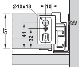
Rear wooden panel installation dimensions
