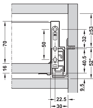
Internal installation height
