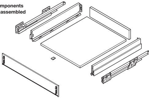
Internal drawer front - supplied assembled but not fitted to drawer
