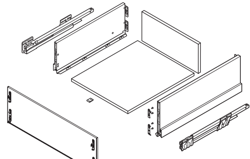
Drawer components - supplied assembled
