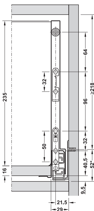
Internal installation height
