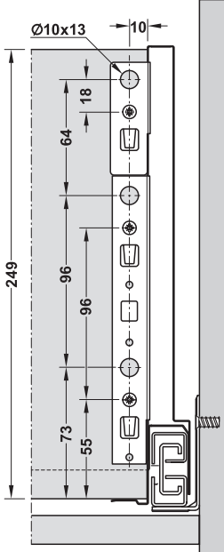
Rear wooden panel installation dimensions
