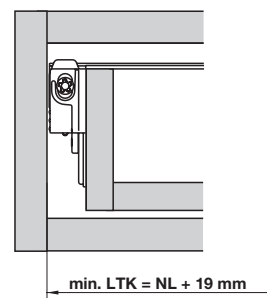
Installation dimensions
