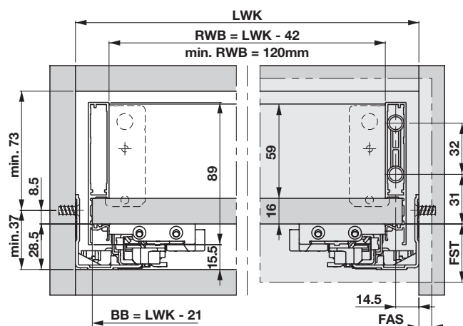
Grass Vionaro Dynapro drawer system, 89 mm high
