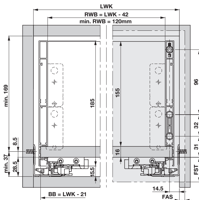
Grass Vionaro Dynapro drawer system, 185 mm high
