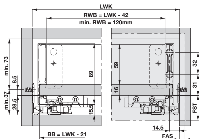
Front panel installation dimensions
