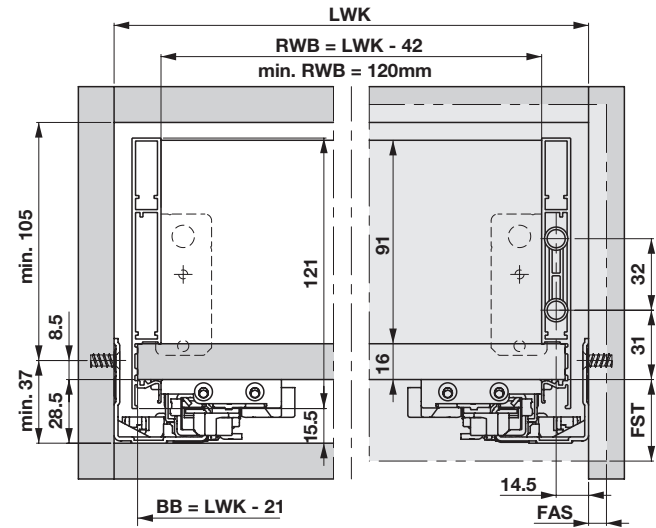
Front panel installation dimensions
