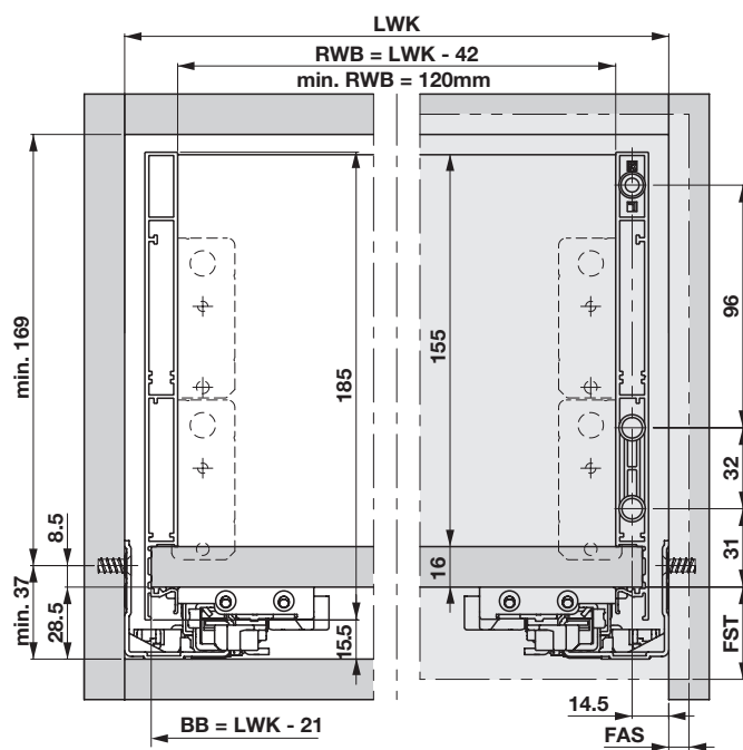
Front panel installation dimensions
