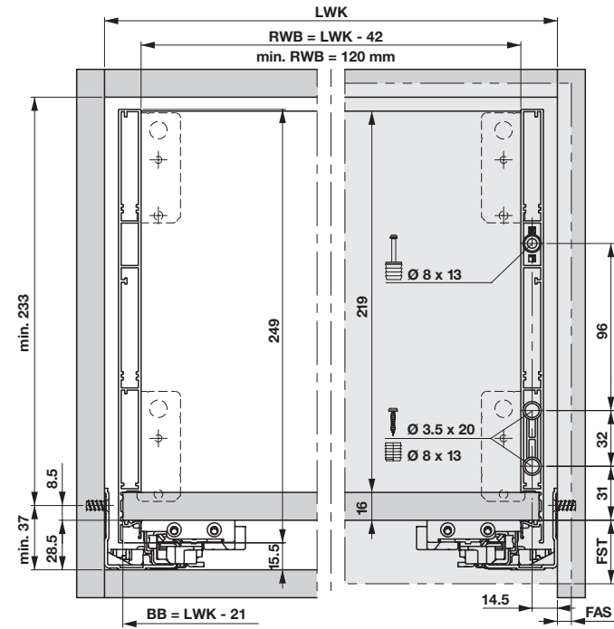
Front panel installation dimensions
